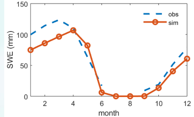
Mean seasonality (1979-2006) of SWE in central Euroasia
